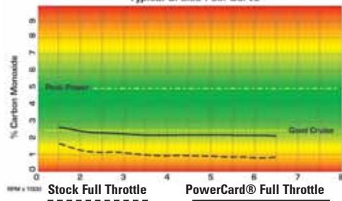
Typical Cruise Fuel Curve
