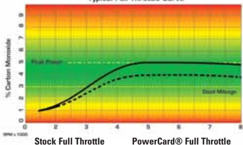
Typical Full Throttle Curve
